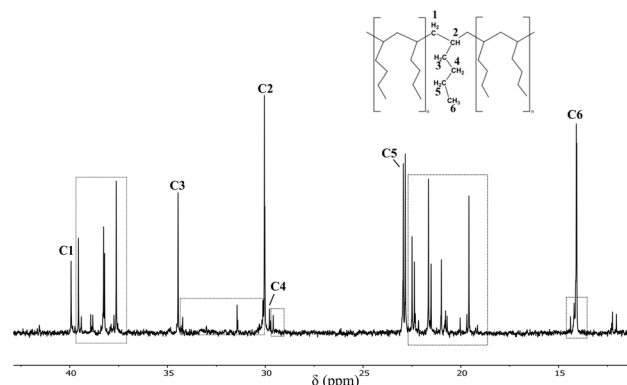
Fig. 5 ^{13}\text{C} NMR (25 ^\circ\text{C} , d-chloroform, 126 MHz) spectrum of poly(1-hexene) prepared using a 10 mol% catalytic loading of 1f at room temperature. # vacuum grease.
