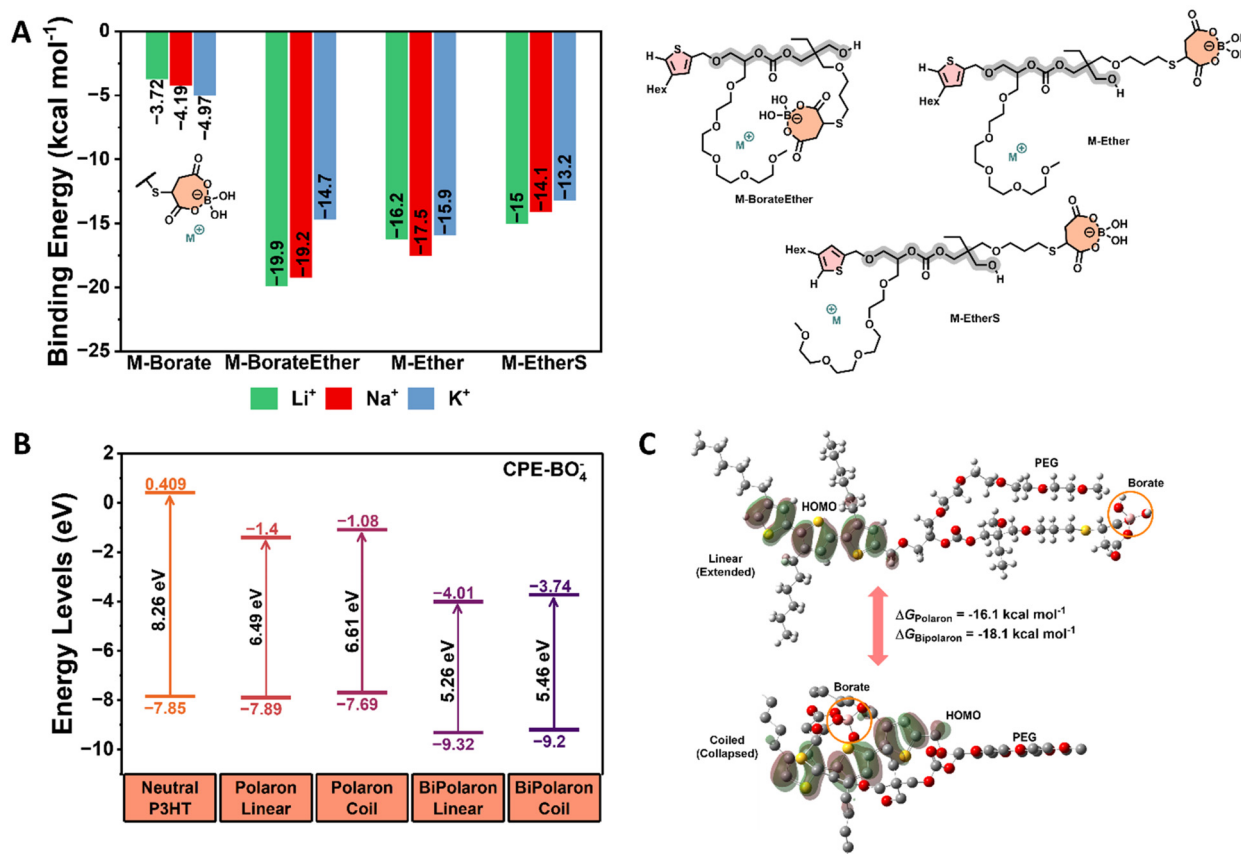
Fig. 6 DFT computations ( \omega B97XD/6-311G(d,p)/cpcm, solvent = DMSO). (A) Cation binding energies in different coordination environments. (B) HOMO–LUMO energies for neutral, polaron, and bipolaron states. Note, for bipolaron systems, the formal HOMO is localised on the borate and hence, the P3HT backbone-localised HOMO–1 is shown for comparison. (C) Relative \Delta\Delta G for coiled and linear conformations with HOMO surfaces for the polaron shown.
