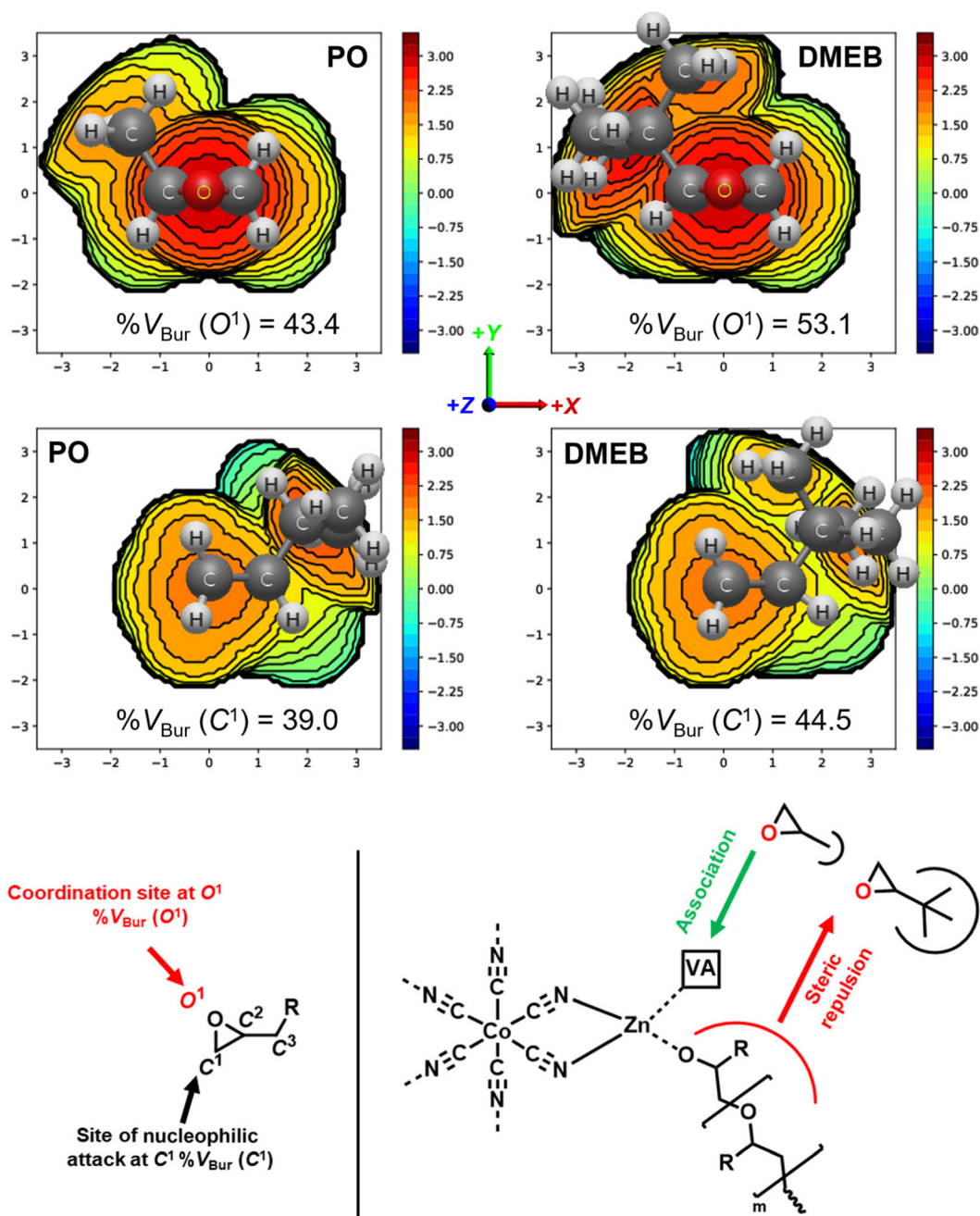
Fig. 4 Top: steric maps of PO and DMEB for the oxygen of the epoxide ring \text{O}^1 and the unsubstituted methylene carbon \text{C}^1 in the direction of the Z-axis. Bottom left: schematic representation of the coordination site and the site of nucleophilic attack. Bottom right: proposed inhibition of DMEB polymerization via DMC catalysis due to steric repulsion.
