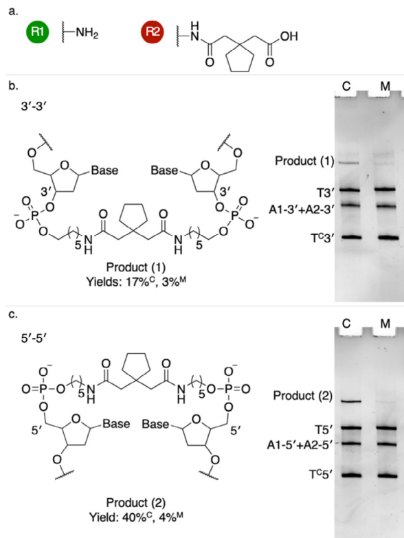
Fig. 2 DNA-templated amide bond formation. (a) Reactive building blocks. (b) Product of reaction across 3'–3' and (c) 5'–5' ends (SI Methods). Strands T C , T C , A1–NH 2 and A2–COOH were annealed in MOPS buffer (pH 7.7) supplemented with MgCl 2 . After annealing then equilibration at 24 °C for 20 h, DMT-MM was added to activate amide coupling (final concentrations: 91 nM T C , 98 nM T C , 99 nM A1–NH 2 , 99 nM A2–COOH, 23 mM MOPS buffer, 18 mM MgCl 2 , 45 mM DMT-MM in a total volume of 35.2 μL). The reaction was run at 25 °C for 20 h. Lane C: fully complementary triplex sequences. Lane M: templating duplex mutated to disrupt triplex formation.
