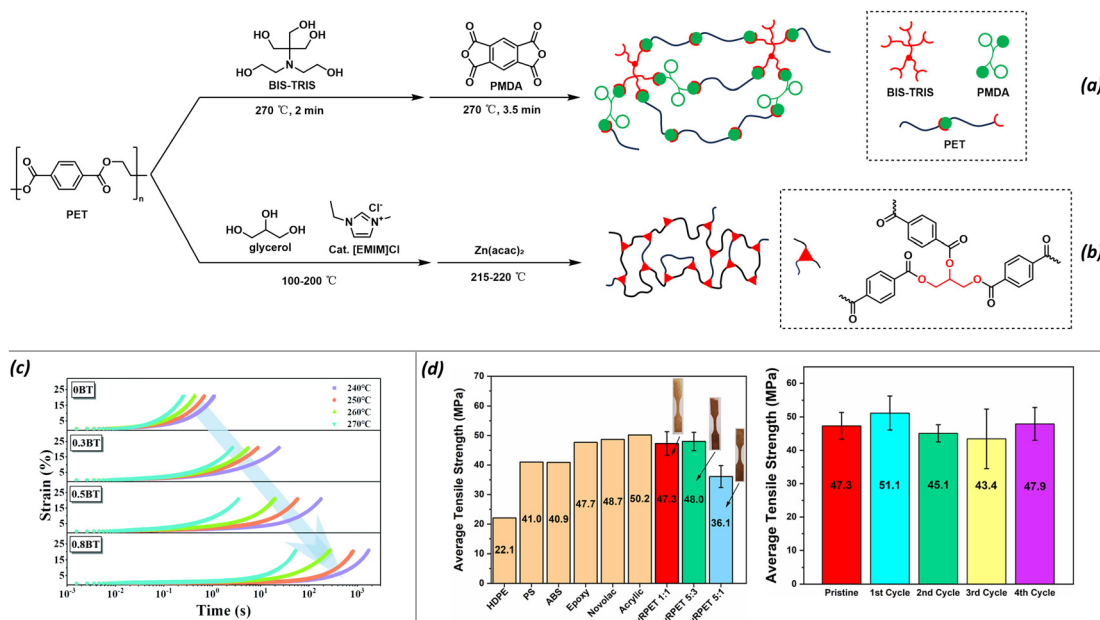
Fig. 12 (a) Synthesis of vitrimers from PET via reactive extrusion with BIS-TRIS and PMDA. (b) Synthesis of vitrimers from PET via glycerol glycolysis and Zn(acac) 2 catalysis. (c) Creep resistance of PET and vitrimers with various BIS-TRIS contents at different temperatures. Reproduced from ref. 61 with permission from Royal Society of Chemistry, copyright 2022. (d) Comparison of mechanical properties between vitrimers with varying glycerol content and common commercial polymers; ultimate tensile strength of the vRPET1:1 sample after 4 cycles shows little change. Reproduced from ref. 35 with permission from Springer Nature, copyright 2023.
