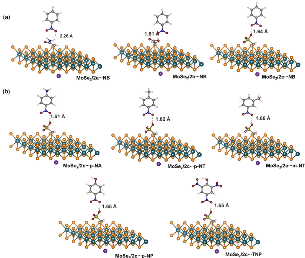
Fig. 3 Relaxed geometries of (a) \text{NB} \cdots \text{MoSe}_2/2\text{a-c} and (b) other NACs interacting with \text{MoSe}_2/2\text{c} showing hydrogen bonds between the acidic O–H from the surface and O=N from the target NACs.
