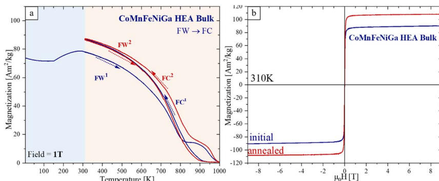
Fig. 11 CoMnFeNiGa HEA bulk: (a) temperature-dependent magnetization at 1 T in the temperature range (5–1000 K); (b) field-dependent magnetization at 310 K before and after annealing ( -9 \text{ T} \geq B_{\text{ext}} \geq 9 \text{ T} ).
