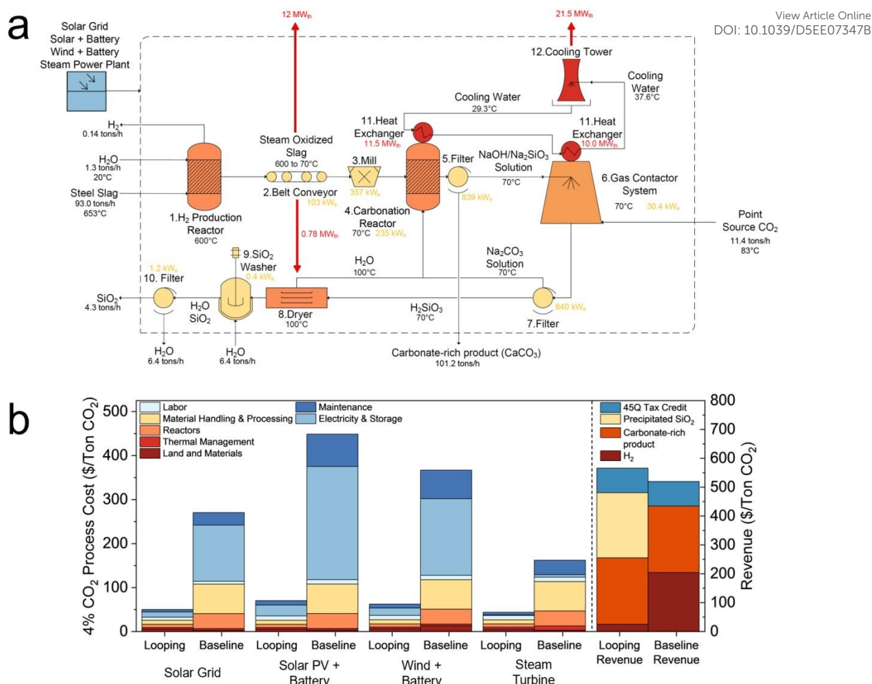
Fig. 3 (a) Proposed plant design for hydrogen (H 2 ) production and point-source CO 2 mineralization through Na 2 CO 3 looping using BOF steel slag. (b) Technoeconomic analysis (TEA) comparing Na 2 CO 3 looping to the baseline process for 4% CO 2 . The process cost was evaluated for different energy (purely electricity) supply methods, including solar grid, internal solar PV with 16-hour battery storage, internal wind turbine with 16-hour battery storage, and an internal steam power plant using waste heat from the slag. The levelized costs of electricity are noted in Table S17. The revenue streams from 45Q tax credit, precipitated silica (SiO 2 ), carbonate-rich product, and H 2 are presented on the right axis.
