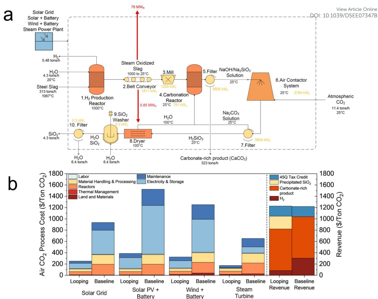
Fig. 4 (a) Proposed plant design for hydrogen (H 2 ) production and air CO 2 mineralization through Na 2 CO 3 looping with BOF steel slag. (b) Technoeconomic analysis (TEA) comparing Na 2 CO 3 looping to the baseline process for 343 ppm CO 2 . The process cost was evaluated for different energy (purely electricity) supply methods, including solar grid, internal solar PV with 16-hour battery storage, internal wind turbine with 16-hour battery storage, and an internal steam power plant using waste heat from the slag. The levelized costs of electricity are noted in Table S17. The revenue streams from H 2 , precipitated silica (SiO 2 ), carbonate-rich product, and the 45Q tax credit are presented on the right axis.
