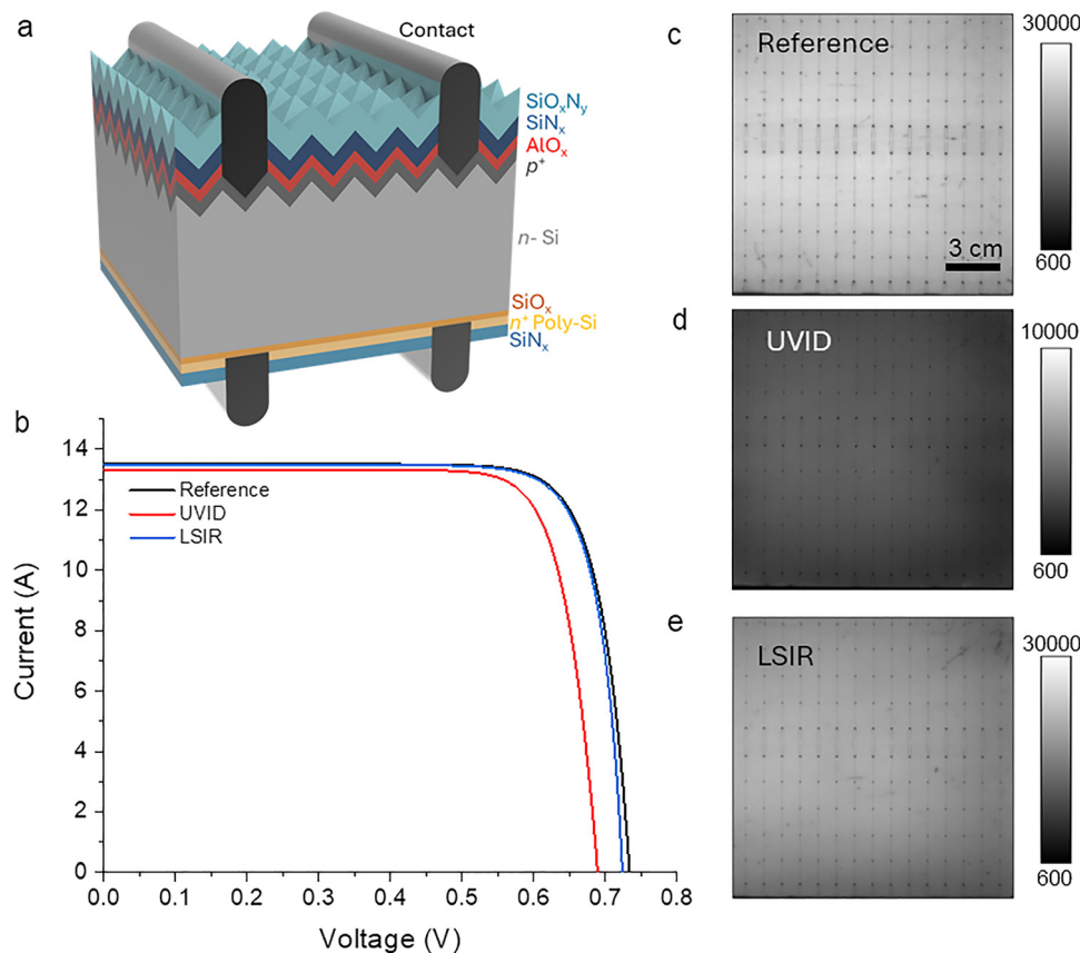
Fig. 1 I - V performance and PL imaging of TOPCon cells after UVID (UV60) and LSIR. (a) Schematic of the device structure of the tested cells. (b) Typical I - V curves of a reference cell and a UVID cell before and after LSIR. (c)-(e) PL images of the TOPCon cells in the original, UVID and LSIR states, respectively, all sharing the same length scale bar as in (c).
