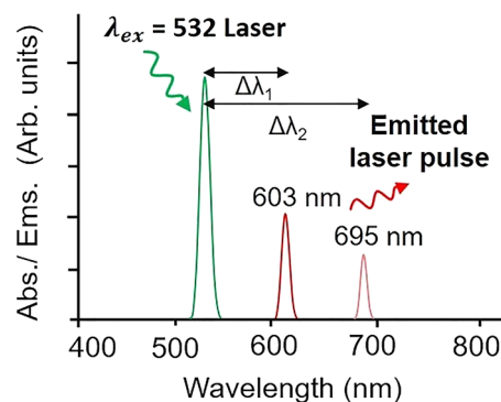
Fig. 9 Illustration of the spectral changes during photon downconversion of the 532 nm laser pulse due to stimulated Raman scattering in an IL; [C_2\text{mim}][\text{dca}] with Raman active dicyanamide anion. Adapted from ref. 105 with permission from [American Physical Society] [Palmer et al., Phys. Rev. Appl. , 2023, 19 , 014052], copyright 2023.
