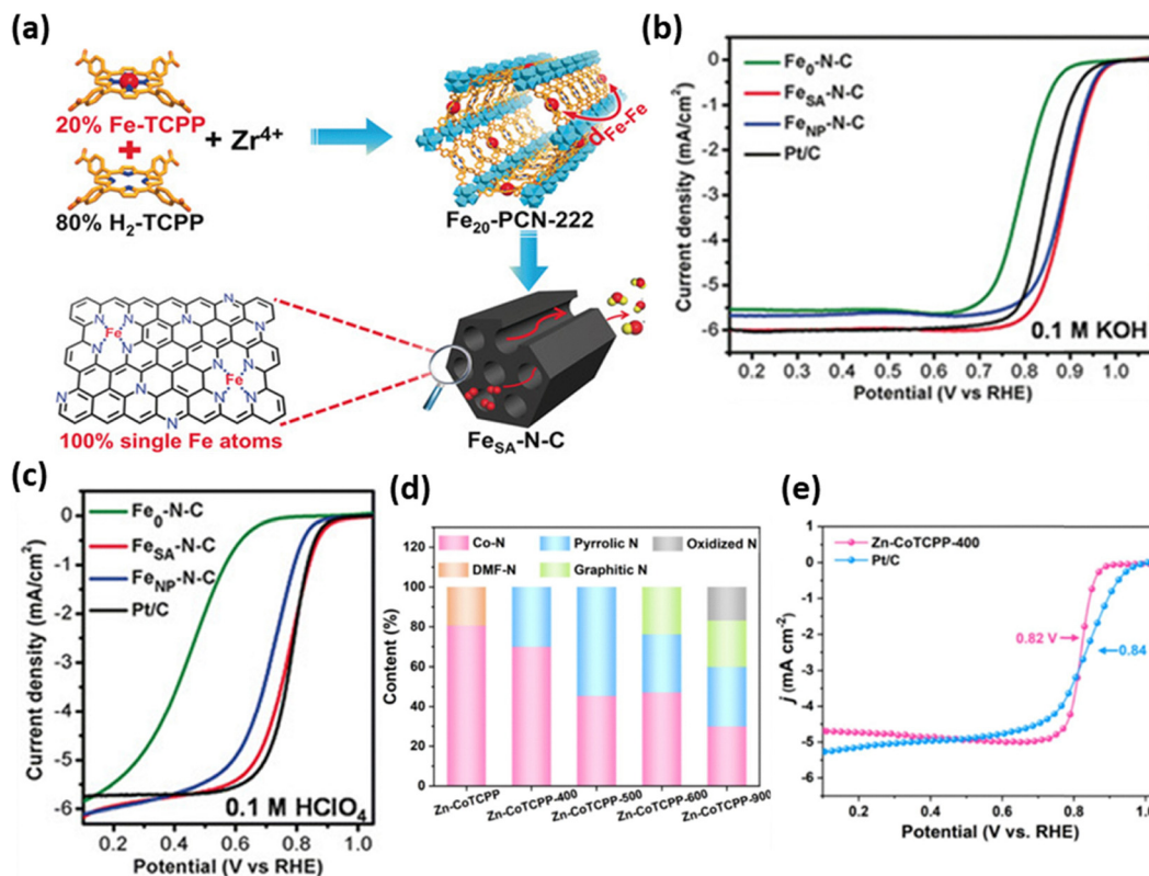
Fig. 5 (a) Schematic representation of the synthetic route for obtaining the Fe–N–C catalyst using MOF-545, including FeTCPP and H 2 TCPP moieties. Linear sweep voltammies obtained for the MOF-545-derived catalysts in (b) alkaline and (c) acidic media. Reproduced from ref. 100 with the permission from John Wiley and Sons, copyright 2018. (d) Normalized content of deconvoluted N-species quantified by high-resolution N 1s XPS. (e) LSV curves for the Zn–CoTCPP-400 electrocatalyst in O 2 -saturated 0.1 M KOH. Reproduced from ref. 101 with the permission from Elsevier, copyright 2025.
