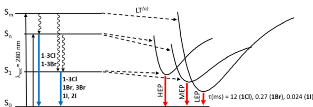
Fig. 14 Comparison through a simplified Jablonski diagram of solid 1-3X . Lifetimes of LEP for 1X are reported. a Even at RT for 1-2I .
