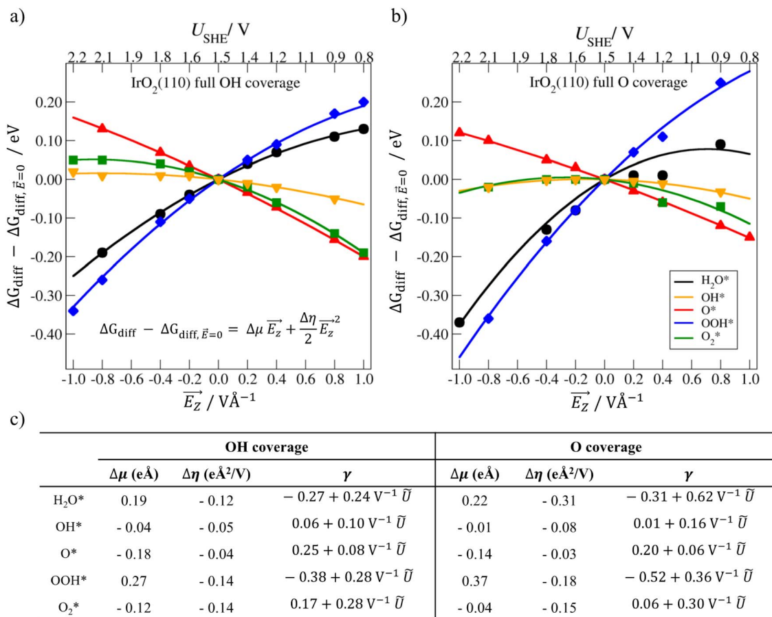
Fig. 3 Field response of the relevant intermediates in OER on \text{IrO}_2(110) under (a) \text{OH}^* coverage and (b) \text{O}^* coverage on \text{Ir}_{\text{CUS}} sites. (c) Table with fitted values for the change in surface dipole ( \Delta\mu, [\text{e}\text{\AA}] ) and polarizability ( \Delta\eta, \left[\frac{\text{e}\text{\AA}^2}{\text{V}}\right] ) associated with a change in surface phase. Additionally, the net potential response for each adsorbate is indicated where \tilde{U} = U_{\text{SHE}} - U_{\text{PZC}} .
