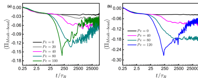
Fig. 9 Plots showing the time evolution of \langle \Pi_{\text{mesh-bead}} \rangle in log-linear scale for (a) K = 30 and (b) K = 50 at \bar{\sigma} = 1.33 .
