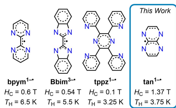
Fig. 1 Selected radical ligands used to construct dinuclear dysprosium single-molecule magnets [(Cp^*_2Dy)_2(\mu-L)]X with coercive fields ( H_C ) and open magnetic hysteresis loops at or below this temperature ( T_H ) under conventional sweep rates. Ligands L are: bpym = 2,2'-bipyrimidine ( X = BPh_4^- ), Bbim = 2,2'-bisbenzimidazole ( X = [K(crypt-222)]^+ , crypt-222 = 2.2.2-cryptand), tppz = 2,3,5,6-tetra(2-pyridyl)pyrazine ( X = BPh_4^- ), tan = 1,4,5,8-tetraazanaphthalene ( X = BArF_{20}^- ).
