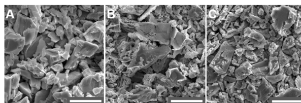
Fig. 1 Plan-view SEM image of (A) Au/CdTe, (B) Au/ZnTe/CdTe, and (C) Au/Cu/ZnTe/CdTe (RTA). Scale bars: 10 \mu\text{m} .
