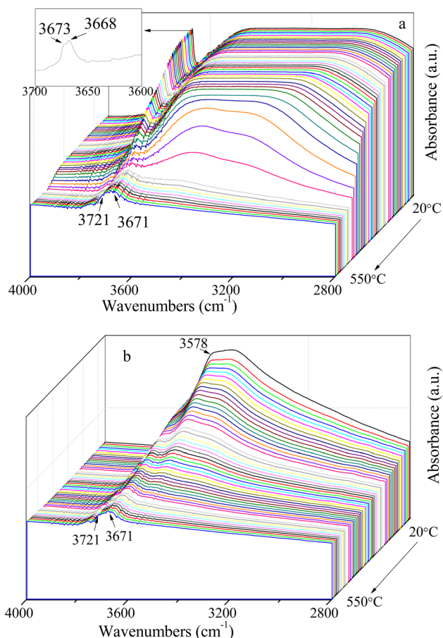
Fig. 7 Change of IR spectra (OH region) of the Au/ \gamma -AlOOH (a) and Au/ \gamma - \text{Al}_2\text{O}_3 (b) as a function of temperature.
