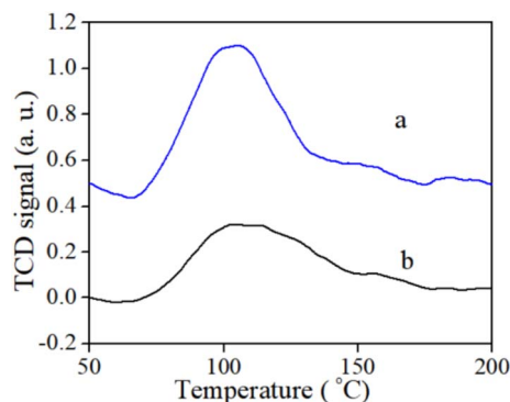
Fig. 6 \text{CO}_2 -TPD profiles of Au/ \gamma -AlOOH (a) and Au/ \gamma - \text{Al}_2\text{O}_3 (b).
