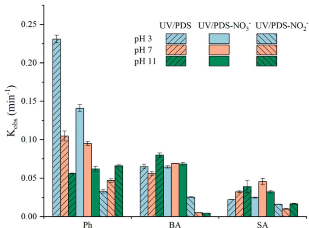
Fig. 2 Effect of pH on reaction rate of the 3 compounds (conditions: [pollutant] = 0.1 mM, [PDS] = 0.5 mM, [\text{NO}_3^-] = 2 \text{ mM} , [\text{NO}_2^-] = 2 \text{ mM} , T = 60 \text{ min} ).
