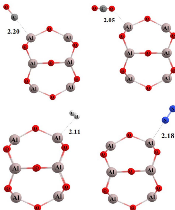
Fig. 4 Optimized structures of gas molecules CO, \text{CO}_2 , \text{H}_2 , and \text{N}_2 adsorbed on the outer surface of the \text{Al}_8\text{O}_{12} cluster. Calculations were performed at the \omega\text{B97XD/Def2-TZVP} level of theory. Bond lengths are presented in Å.
