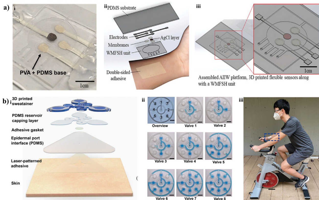
Fig. 18 (a) (i) Image of the AllIW patch integrating 3D-printed ion-sensing electrodes with a wearable microfluidic sample-handling module. (ii) Breakdown of the AllIW patch showing individual elements. (iii) Diagram displaying the layout of AllIW patch components both prior to and after final assembly. Reproduced with permission from ref. 224. Copyright 2021, Wiley. (b) (i) schematic illustrating the main parts of the sweatainer platform and its interface with skin, produced using DLP printing. (ii) time-lapse sequence showing fluid entry into various chamber-by-volume designs in a specific order. (iii) Image of the sweatainer device adhered to a user's skin during physical activity. Reproduced with permission from ref. 228. Copyright 2023, AAAS.
