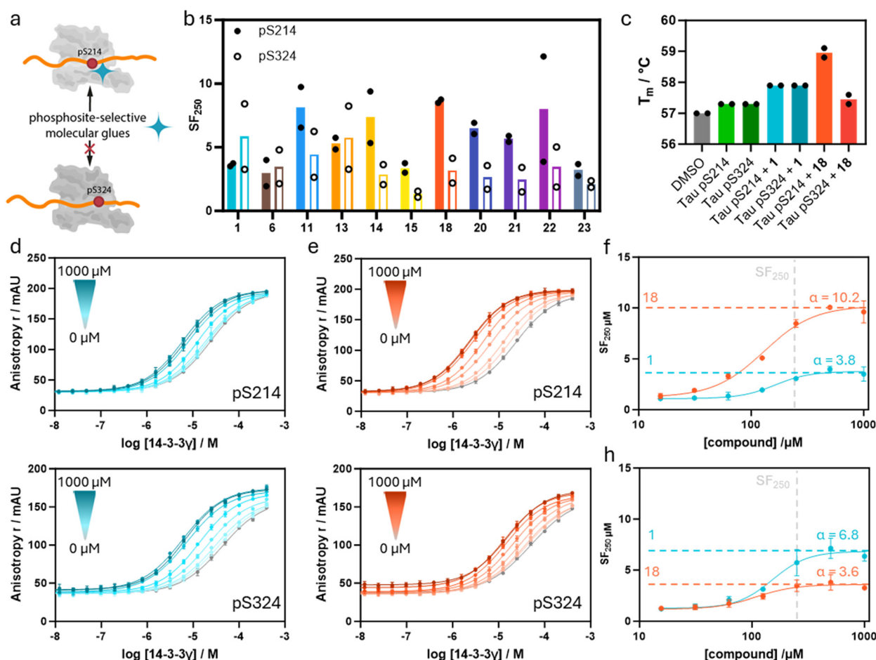
Fig. 5 a Phospho-site selective 14-3-3/Tau PPI stabilization. b SF_{250\mu M} of selected compounds for stabilization of the 14-3-3 \gamma complex with Tau pS214 and Tau pS324 peptides based on the internal DMSO reference. Mean of two separately performed experiments (see ESI† Fig. S9 for the corresponding binding curves). c Differential scanning fluorimetry assay results. Identified melting temperatures ( T_m ) of 14-3-3 \gamma in the presence of the Tau pS214 or pS324 peptide and compounds 1 and 18 . Mean of two separately performed experiments. d and e 14-3-3 \gamma titrations in the presence of increasing concentrations of compounds 1 (d) and 18 (e), in the presence of either 100 nM fluorescein-labeled Tau pS214 or fluorescein-labeled Tau pS324. Overnight measurement, mean and SD of scientific duplicate. f, SF_{250\mu M} of the 14-3-3 \gamma /Tau pS214 interaction plotted against compound concentrations. The data are derived from 2D titrations (d and e). The saturation of the ratio represents the \alpha -factor. (h) Ratio of K_D /apparent K_D of the 14-3-3 \gamma /Tau pS324 interaction plotted against compound concentrations. The data are derived from 2D titrations (figures d and e). The saturation of the ratio represents the \alpha -factor.
