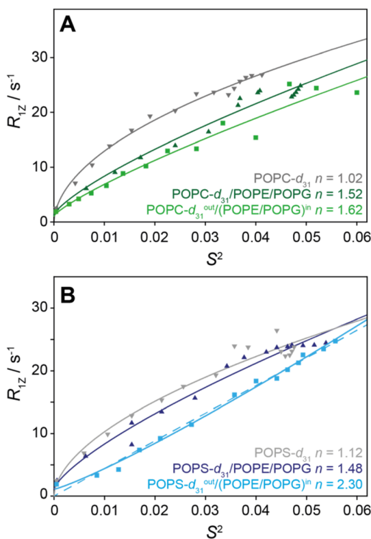
Fig. 3 (A) Square law plots of POPC- d_{31}^{out}/(POPE/POPG)^{in} membranes (light green squares), symmetric POPC- d_{31} /POPE/POPG bilayers (dark green triangles), and pure POPC- d_{31} membranes (gray upside down triangles). (B) Square law plots of POPS- d_{31}^{out}/(POPE/POPG)^{in} membranes (light blue squares), symmetric POPS- d_{31} /POPE/POPG bilayers (dark blue triangles), and pure POPS- d_{31} membranes (light gray upside down triangles). The lines represent best fits to the function R_{1Z} = y_0 + a \times S^n , and the dashed solid line represents a linear regression.
