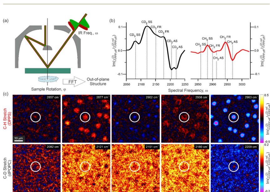
Fig. 1 Azimuthal-scanned phase-resolved SFG microscopy of a mixed lipid monolayer of 1 : 1 DPPS : dPOPC. (a) Schematic of the SFG microscope. (b) Imaginary parts of the out-of-plane spectra averaged over the entire image, in both the C–D (black) and C–H (red) frequency ranges, with labels showing the assignment of the resonant features. (c) Images at selected frequencies through the two frequency ranges. A single condensed lipid domain is encircled in each image for reference. All SFG spectra and images are from the PPP polarisation combination and are given relative to the response from a z-cut quartz reference.
