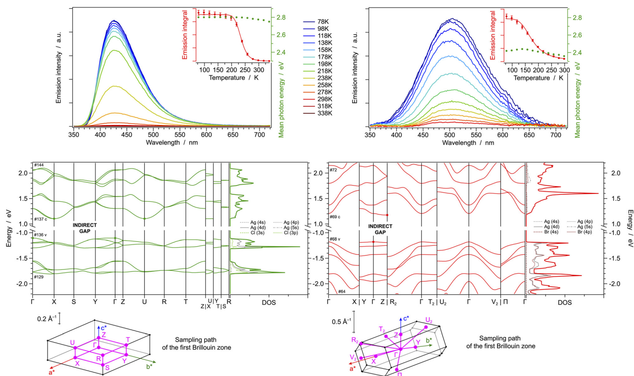
Fig. 2 (Top) Temperature-dependent emission spectra of [(\text{AgCl})(2\text{-pica})]_n (left) and [(\text{AgBr})(2\text{-pica})]_n (right), measured in the range between 78 and 338 K; the change in the emission intensity and mean-photon energy is also reported in the graph inset. (Bottom) Band-structure diagram and density-of-states (DOS) plot with relative orbital contributions; the band-structure path in the reciprocal space is also depicted.
