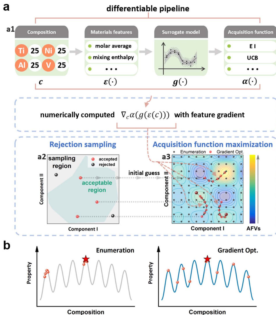
Fig. 1 Schematic pipeline of the proposed BO strategy for composition design, utilizing feature gradient, \nabla_c \alpha(g(\varepsilon(c))) , to efficiently maximize AFs. (a) The complete differentiable pipeline, \nabla_c \alpha(g(\varepsilon(c))) , linking alloy compositions (values represent atomic percentages in a1)), material features, GPR predictions, and AF values (AFVs). AF maximization in (a3) is achieved efficiently using the gradient information, with a rejection sampling step in (a2) to generate feasible initial compositions, ensuring they fall within the desired design space. (b) Illustration showing that this gradient-based approach yields a broader set of candidate compositions by identifying multiple distinct local maxima, as opposed to traditional enumeration-based methods which tend to focus on a narrower set of options. This results in more balanced exploration of the compositional space, rather than strict exploitation of a single optimum.
