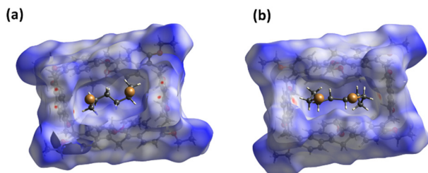
Fig. 7 Hirshfeld surfaces (mapped with d_{norm} ) illustrating the interaction modes presented from the top view of [PS-6 \supset DBH] (a) and of [PS-6 \supset DBO] (b).
