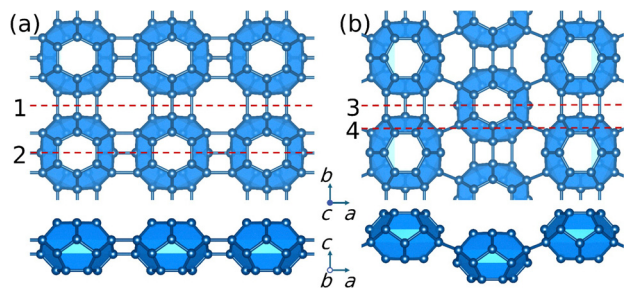
Fig. 12 Top and side views of crystal structures of (a) qTP and (b) qHP C 24 monolayers. 92
