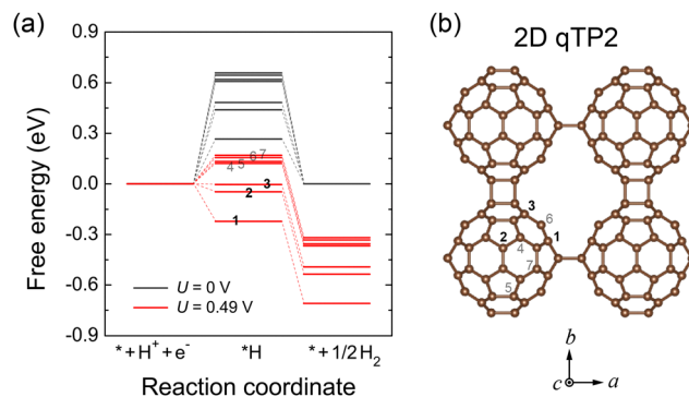
Fig. 9 (a) Gibbs free energy changes associated with the HER in qTP2 C_{60} networks at a pH of 0 and room temperature. (b) Adsorption sites for qTP2 C_{60} networks, with lower to higher numbers corresponding to lower to higher free energies of the intermediates. 91
