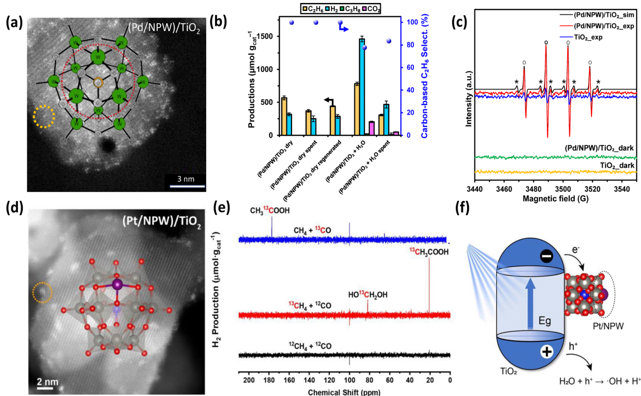
Fig. 6 (a) STEM-HAADF images of (Pd/NPW)/TiO 2 . Color code: O – white, P – orange, W – green. (b) Methane photocatalytic coupling on (Pd/NPW)/TiO 2 nanocomposites in dry and aqueous environments. (c) EPR spectra of DMPO spin trapping of (Pd/NPW)/TiO 2 and TiO 2 under methane, *Signals of DMPO/ \bullet\text{CH}_3 , *Signals of DMPO/ \bullet\text{OH} . 37 Reproduced from ref. 37 with permission from Elsevier, copyright 2024. (d) Atomic-resolved HAADF-STEM image of Pt/NPW/TiO 2 (3 : 10). The inset image represents the monomer of Keggin-structured NPW with isolated Pt atoms anchored at the 4-fold hollow site of W–O–W, color code: red (oxygen), gray (tungsten), blue (phosphorus), purple (platinum). (e) 13 C NMR spectra of liquid products of (Pt/NPW)/TiO 2 (3 : 5) with 12 CH 4 + 12 CO, 13 CH 4 + 12 CO, and 12 CH 4 + 13 CO. (f) Scheme of the generation of photoexcited charge carriers by Pt/NPW. 104 Reproduced from ref. 104 with permission from American Chemical Society, copyright 2023.
