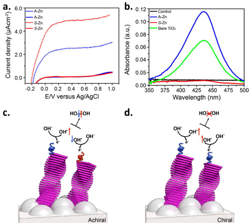
Fig. 1 Spin-specific electron transfer and its impact on photocurrent density and peroxide formation. (a) Photocurrent density comparison of TiO 2 electrodes coated with self-assembled molecules. Achirality is presented by the blue line, whereas chirality is represented by the red line. (b) The UV-vis absorption spectra of the neutral electrolyte solution (0.1 M Na 2 SO 4 ) titrated with o -tolidine while using bare TiO 2 and Zn-porphyrin-coated TiO 2 (achiral A-Zn or chiral S-Zn) working electrodes. (c) When the anode does not exhibit spin-selectivity, OH• radicals have antiparallel spins, interacting on a singlet surface that produces H 2 O 2 . (d) Conversely, spin-specific electron transfer aligns the spins parallelly, leading to interaction on a triplet surface that prevents H 2 O 2 formation and promotes ground-state oxygen production. Figures adopted from ref. 8 with permission from American Chemical Society © 2017.
