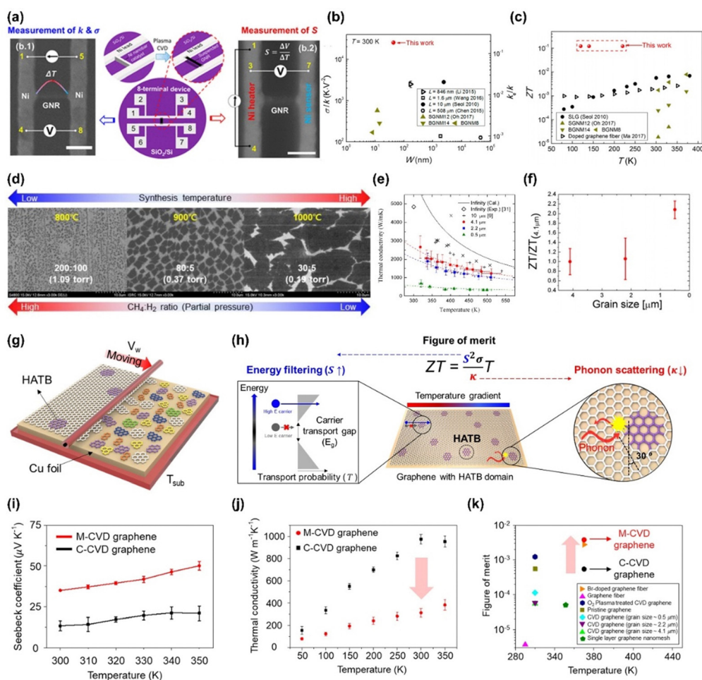
Fig. 3 (a) Test structure for the thermoelectric measurements of the GNR grown via CVD. (b) \sigma/k and S/k ratios of the suspended GNR compared with reference data. (c) zT value of the suspended GNR compared with reference data. Reproduced with permission from ref. 45. (d) Scanning electron microscopy (SEM) images of different nucleation densities in the initial growth state depending on the synthesis temperature and pressure. (e) Thermal conductivity as a function of temperature for different grain sizes. Reproduced with permission from ref. 31. (f) zT value of the graphene with the optimized grain size. Reproduced with permission from ref. 48. (g) Growth mechanism of MHW-CVD graphene. (h) Concept of increasing the graphene zT value in the MHW-CVD system. (i) Comparison between the Seebeck coefficients of M-CVD and C-CVD graphene. (j) Comparison between the thermal conductivities of M-CVD and C-CVD graphene. (k) zT values of M-CVD and C-CVD graphene compared with reference data. Reproduced with permission from ref. 13.
