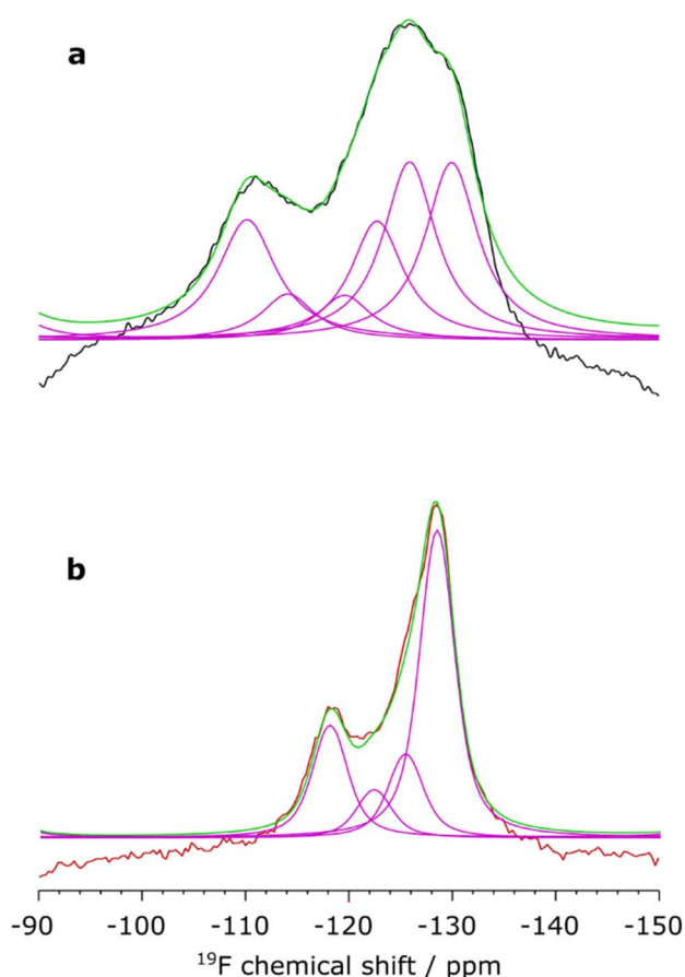
Fig. 3 20 T \{^1\text{H}\}\text{--}^{19}\text{F} CPMAS NMR spectra recorded with cooling ( \sim 260\text{ K} ) and using a MAS frequency of \sim 33\text{ kHz} . Spectra shown are of (a) 3FP-dosed zeolite HY (black) and (b) 3FP-dosed HZSM-5 (red), with deconvolutions (purple) and the envelope (green). Fitted parameters are given in Table S10 † .
