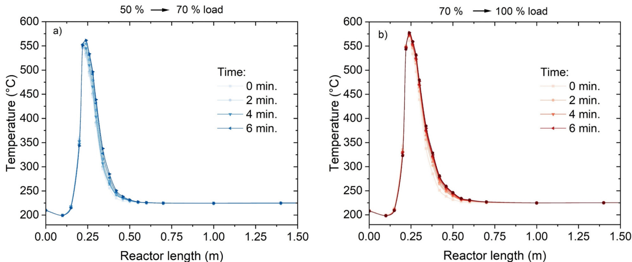
Fig. 8 Temperature profiles during the load variation: (a) from 50 to 70% load; (b) from 70 to 100% load (experimental conditions: 8 bar, \text{H}_2 : \text{CO}_2 = 4.15 , cooling setpoint = 230 °C).
