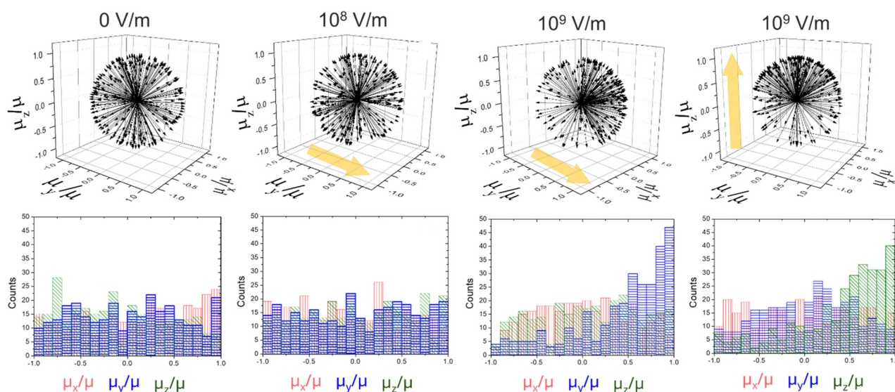
Fig. 4 Representation of the normalized dipole moment components of the 300 molecules in the MD vapor-deposited glasses for TPD-Br1 prepared at 300 K and under 0, 10^8 and 10^9 V m ^{-1} electric fields along \hat{y} (in plane) and \hat{z} (out of plane) (direction of the field in yellow). The histograms show the counts of the normalized projections: \mu_x/\mu (in orange, vertical lines) \mu_y/\mu (in blue, horizontal lines) and \mu_z/\mu (in green, diagonal lines) of each specific case.
