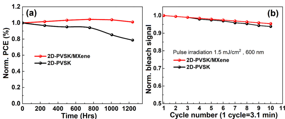
Fig. 6 (a) Stability of the PCE under open-air conditions and (b) photostability under fs pulse excitation for pristine and MXene-passivated PSC. The pump pulse was 1.5 \text{ mJ cm}^{-2} at 600 nm, and TA amplitude at 712 nm and fixed time delay at 6 ps after excitation (maximum of the bulk bleach signal) is taken to monitor the photodegradation.
