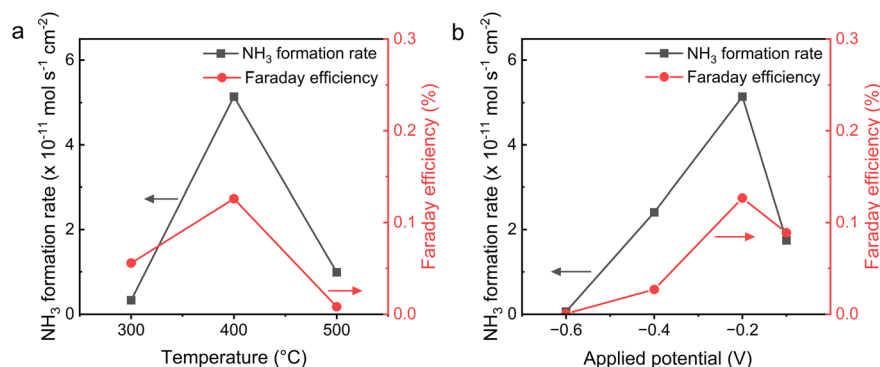
Fig. 5 NH 3 formation rate and Faraday efficiency of the I-Ru-LSCF-BZCYYb|BZCYYb|Ni-BZCYYb electrolysis cell (a) at different temperatures and an applied potential of -0.2 V, and (b) at 400 °C and different potentials. Reaction gas: pure \text{N}_2 at the working electrode; 5% \text{H}_2 –95% Ar at the counter electrode (reference electrode).
