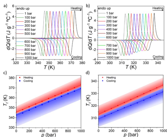
Fig. 5 VT-DSC curves at different pressures for (a) compound 1 and (b) compound 2 . Transition temperature dependence with pressure for (c) compound 1 and (d) compound 2 . Note: solid points indicate the peak maximums, solid lines represent, and shaded areas represent the peak width from the onset to the offset of the peaks. Red = heating data, blue = cooling data.
