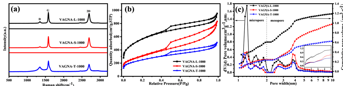
Fig. 4 (a) Raman spectra, (b) nitrogen adsorption-desorption isotherms and (c) pore size distributions (PSDs) of VAGNA-L-1000, VAGNA-S-1000 and VAGNA-T-1000.
