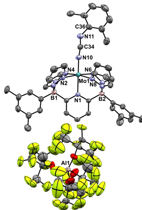
Fig. 6 Molecular structure of [\mathbf{4-Xyl}]^+ . Thermal ellipsoids are shown at the 50% probability level and all H atoms are omitted for clarity. Selected bond distances (Å): \text{Mo(1)-N(1)} , 2.167(3) ; \text{Mo(1)-N(10)} , 1.921(3) ; \text{N(10)-C(34)} , 1.210(5) ; \text{C(34)-N(11)} , 1.207(5) ; \text{N(11)-C(36)} , 1.391(6) selected bond angles ( ^{\circ} ): \text{N(1)-Mo(1)-N(10)} , 176.82(12) ; \text{Mo(1)-N(10)-C(34)} , 171.8(3) ; \text{N(10)-C(34)-N(11)} , 170.1(5) ; \text{C(34)-N(11)-C(36)} , 137.1(4) .
