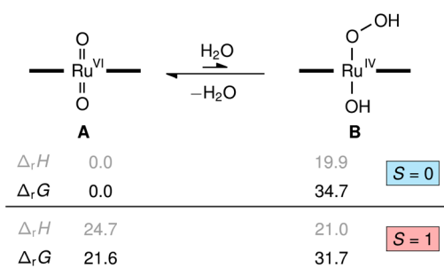
Fig. 9 Relative enthalpies and Gibbs free energies in \text{kcal mol}^{-1} for the formation of [(\text{L}1)\text{Ru}^{\text{IV}}(\text{OH})(\text{OOH})] , B , from [(\text{L}1)\text{Ru}^{\text{VI}}(\text{O})_2] , A , and water computed at the M06L-D3(SMD)/def2-TZVP level (porphyrin ligand L1 illustrated with horizontal bars).
