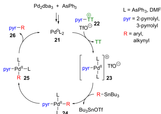
Scheme 11 Proposed mechanistic cycle for pyrrolysulfonium Stille couplings.
