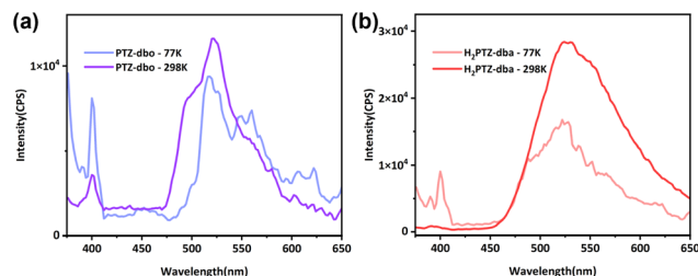
Fig. 3 (a) Solid PL spectra of PTZ-dbo at different temperatures; (b) solid PL spectra of \text{H}_2\text{PTZ-dba} at different temperatures.
