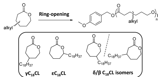
Scheme 1 General scheme for the ring-opening polymerisation of n -alkyl-substituted \varepsilon -caprolactone monomers.
