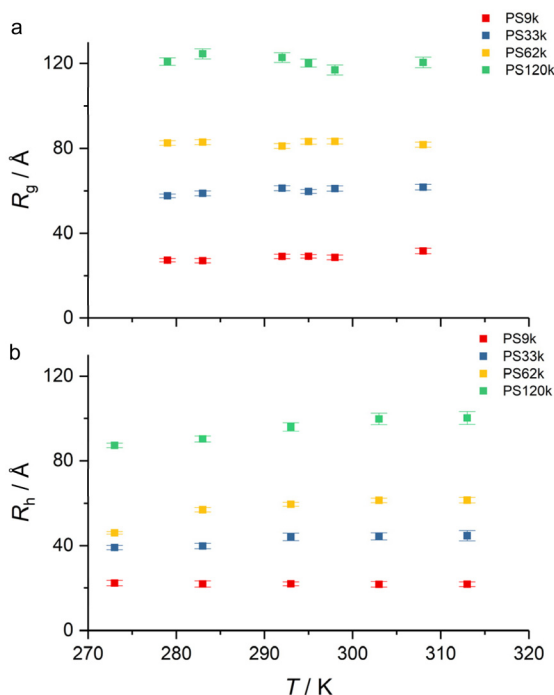
Fig. 4 Comparison of (a) R_g gathered from SANS data fittings and (b) R_h gathered from DOSY-NMR (obtained using dsteppgp3s) applied to the Stokes–Einstein equation of the polystyrene standard (average molar masses of 9, 33, 62 and 120 kg mol −1 ).
