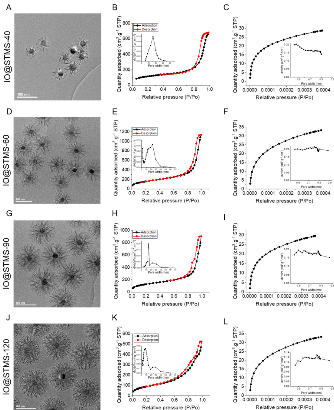
Fig. 7 TEM images (issued from Fig. 6, Fig. S6 and S7 † ), adsorption–desorption isotherms at high relative pressures including an inset with the BJH desorption pore volume plot, and adsorption isotherms at small relative pressures including an inset with the Horvath–Kawazoe differential pore volume plot for IO@STMS-40 (A–C), IO@STMS-60 (D–F), IO@STMS-90 (G–I) and IO@STMS-120 (J–L).
