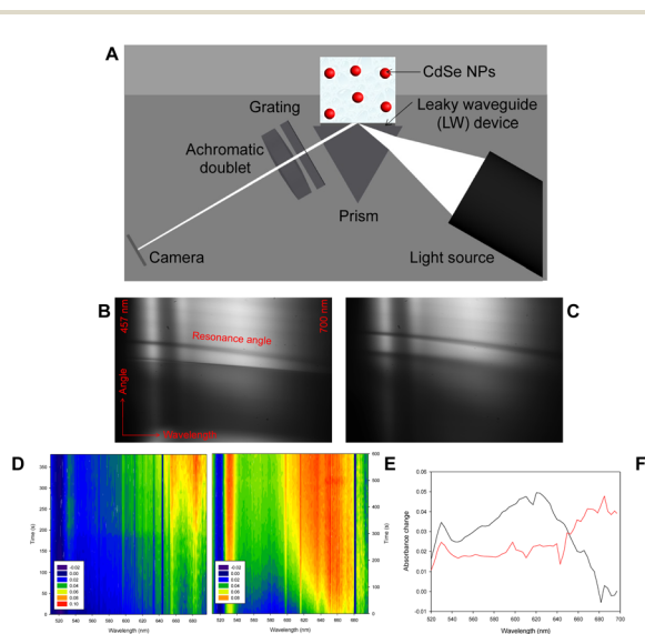
Fig. 5 (A) Scheme of leaky waveguides (LWs) for monitoring; 2D reflectivity curves of a LW with chemically formed NP suspension at time (B) 0 s and (C) 300 s; absorbance versus wavelength and time obtained using LW spectroscopy for (D) chemically and (E) bioelectrochemically synthesised NPs; (F) absorbance change measured using LW spectroscopy from 0 to 300 s for chemically (red curve) and from 0 to 600 s for bioelectrochemically (black curve) formed NPs.
