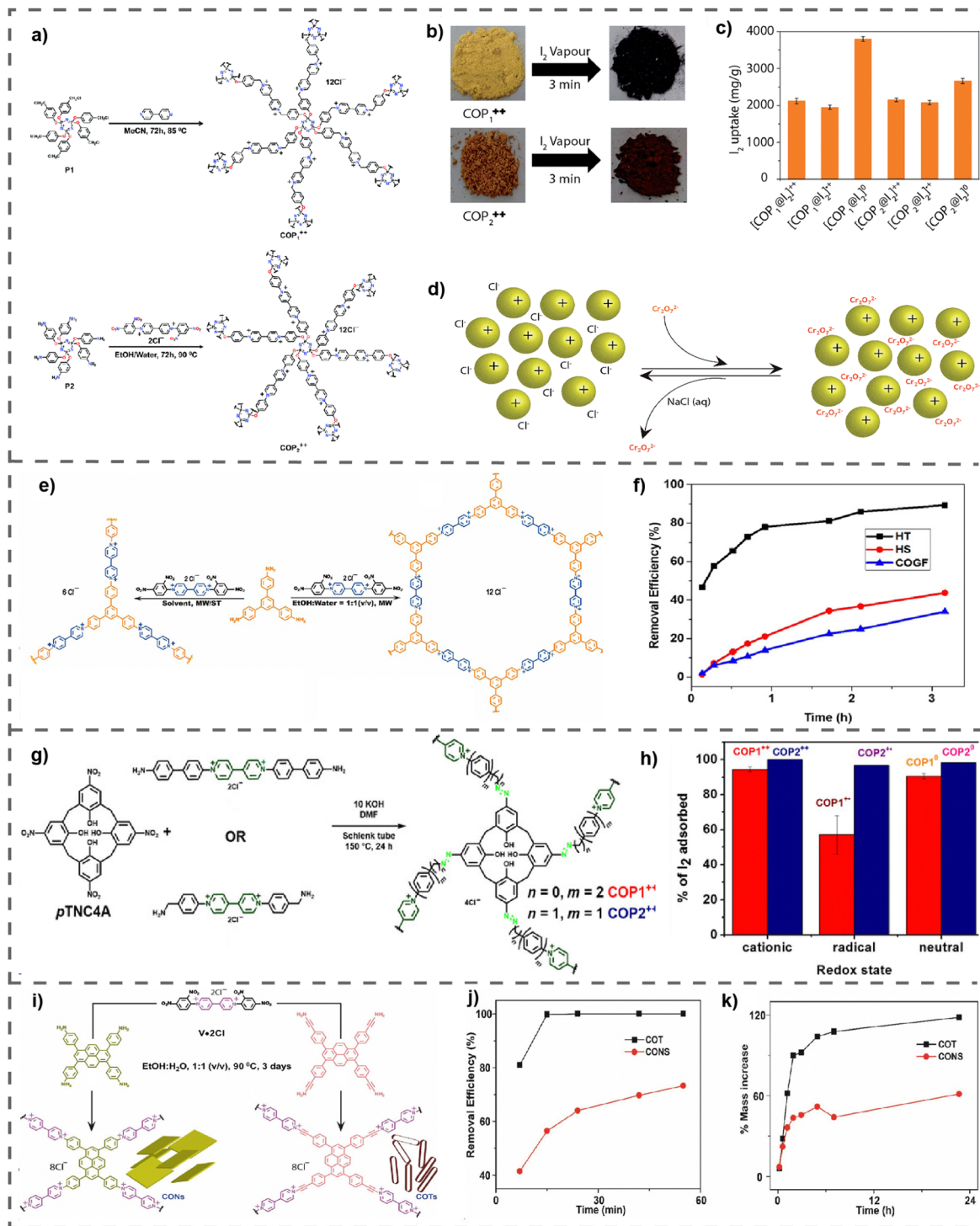
Fig. 5 (a) Synthesis of COP 1 1+ and COP 2 1+ . (b) Real images of iodine vapor adsorption in COP 1 and COP 2 at 60 °C. (c) Iodine vapor capture capacities of COP 1 and COP 2 in three different redox states. (d) Schematic representation of anion removal (MnO 4 - , Cr 2 O 7 2- ) by anion exchange, where yellow spheres represent polymer particles (COP 1 and COP 2 ). Reproduced with permission from ref. 70. Copyright 2014 the Royal Society of Chemistry. (e) Synthesis of the hollow sphere (HS) and hollow tube (HT) via the solvothermal synthesis approach and the covalent organic gel framework (COGF) via the microwave synthesis approach. (f) Graph of % removal of I 2 from a 1 mM solution in cyclohexane over time by HT, HS and COGF. Reproduced with permission from ref. 43. Copyright 2022, American Chemical Society. (g) Synthesis of COP 1 1+ and COP 2 1+ . (h) Solution-phase iodine adsorption by the three redox states of COP 1 and COP 2 . Reproduced with permission from ref. 69. Copyright 2022 Wiley-VCH. (i) Synthesis of CONs and COTs, (j) and (k) iodine adsorption experiments. Reproduced with permission from ref. 89. Copyright 2022 Wiley-VCH.
