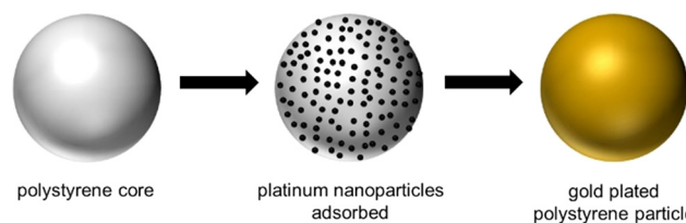
Fig. 1 Graphical schematic depicting the synthetic steps of the addition of a gold shell to a polystyrene core particle.
