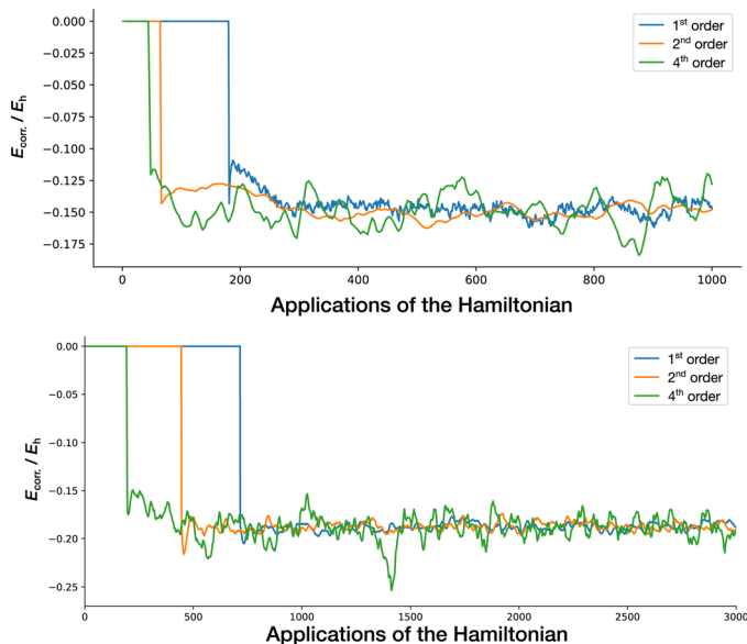
Fig. 9 The top panel shows an MR-CCMCS propagation for \text{Be}_2/\text{cc-pVQZ} at 2.5 \text{ \AA} separation with the (4e,8o) CAS reference space run with the first-, second- and fourth-order Chebyshev projectors. The bottom panel shows an i-FCIQMC propagation of \text{Be}_2/\text{cc-pVTZ} at 2.5 \text{ \AA} separation, using the same propagators. Here we only show the shift as an estimator for E_{\text{corr}} for clarity.
