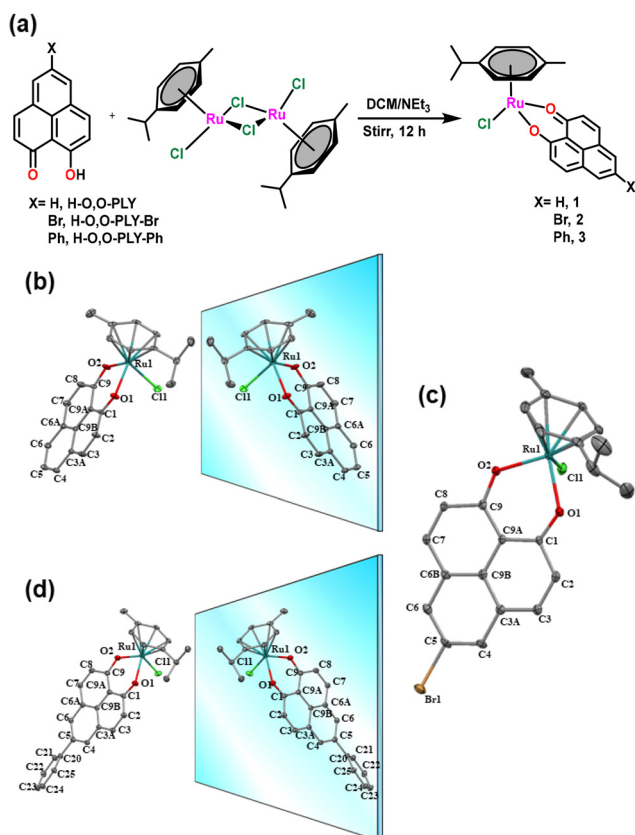
Fig. 1 (a) Synthetic scheme of complex 1–3 . (b–d) Perspective view of complex 1–3 with 50% thermal ellipsoidal probability. All the hydrogen atoms are omitted for clarity.
