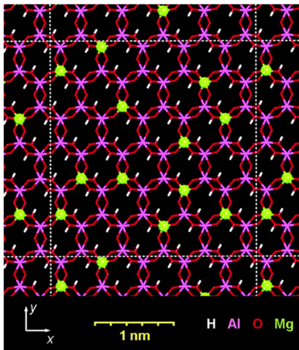
Fig. 18 Octahedral layer of \text{Na}_{0.8}[\text{Si}_8]^{\text{IV}}[\text{Al}_{3.2}\text{Mg}_{0.8}]\text{VO}_{20}(\text{OH})_4 viewed normal to the surface. The average distribution of Mg defects (highlighted) is shown. Four types of “defect” distribution: (1) a total of 35% of the Al atoms is surrounded by three Al atoms and no Mg; (2) 55% of the Al atoms is surrounded by two Al atoms and one Mg atom; (3) 10% of the Al atoms is surrounded by one Al atom and two Mg atoms; and (4) none of the Al atoms are surrounded by three Mg neighbours. Reprinted with permission from ref. 377. Copyright 2005, the American Chemical Society.
